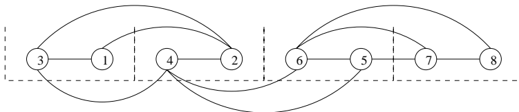
Figure 4: After running the perfect matching algorithm, we get a layout with maximum distance at most 3 \leq 2B(G) .
